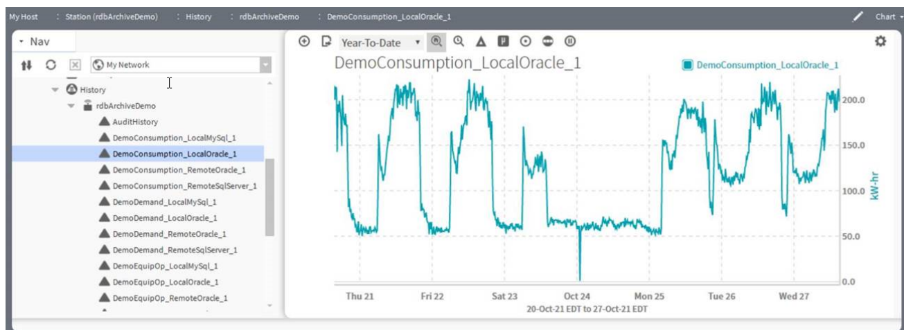
Figure 13 Local data
