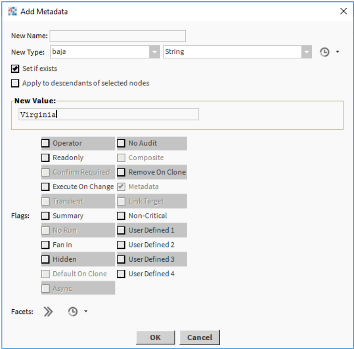
Figure 60 Metadata window
