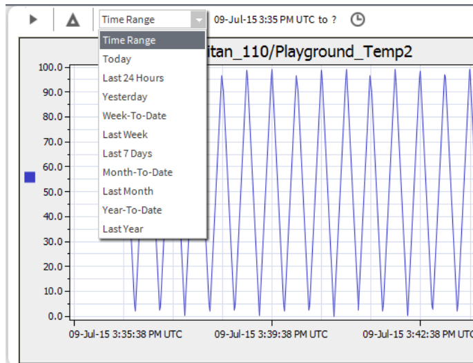
Figure 41 HistoryChart view
